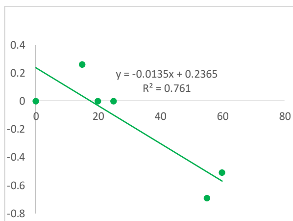
Fig 9: showing first-order kinetics
