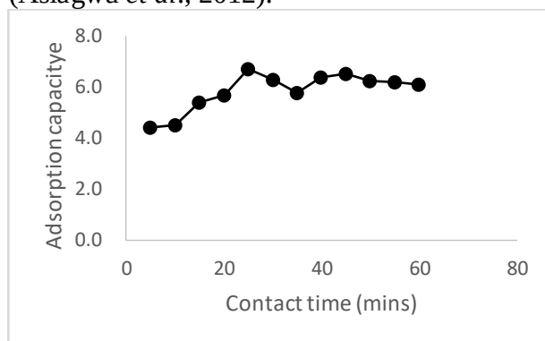
Fig. 4: Effect of contact time on tartrazine dye removal with activated silica
