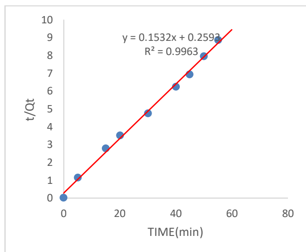
Fig 10: showing second-order kinetics
