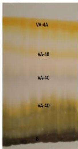
Plate 1: TLC Plate of Ethylacetate Extract of Leaves of Vernonia amygdalina (Fraction 4) Developed using Hexane: Ethyleacetate: Methanol (3:2:2). 4A-4D = Sub fractions of VA-4, B = Origin
